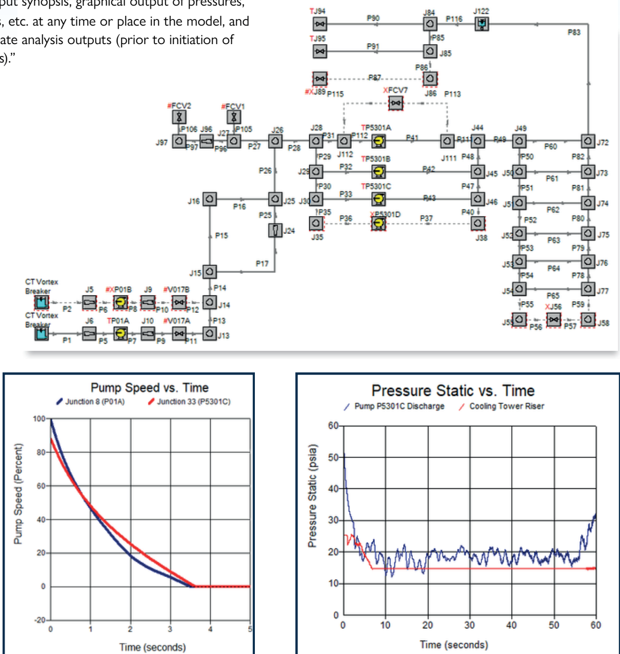
Pump speed vs. time graph for one of the existing circulating pumps and one of the new booster pumps after tripping
