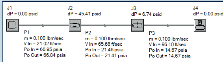
FIGURE 1: Dacacor Arrow model of a sonic venturi system
