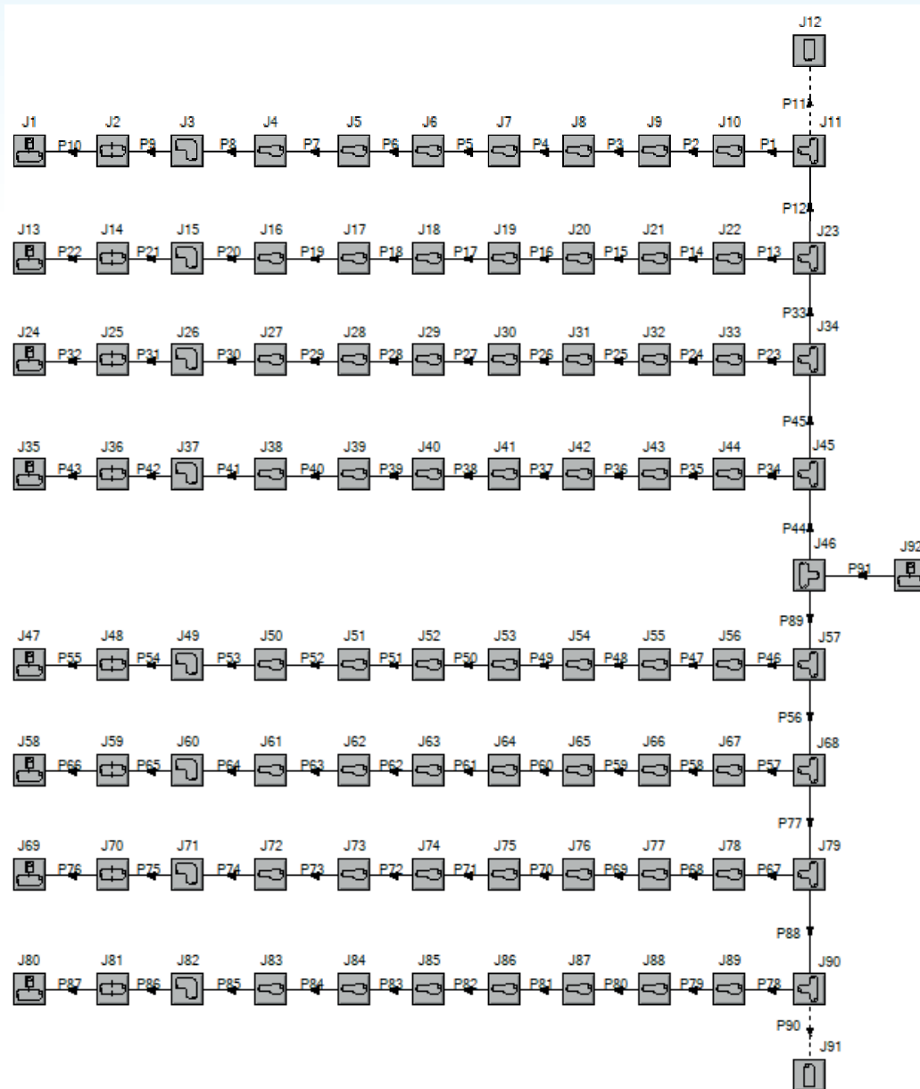
FIGURE 1: Dacacor Arrow model of a Rolls Royce Avon gas turbine for a power generation application.
